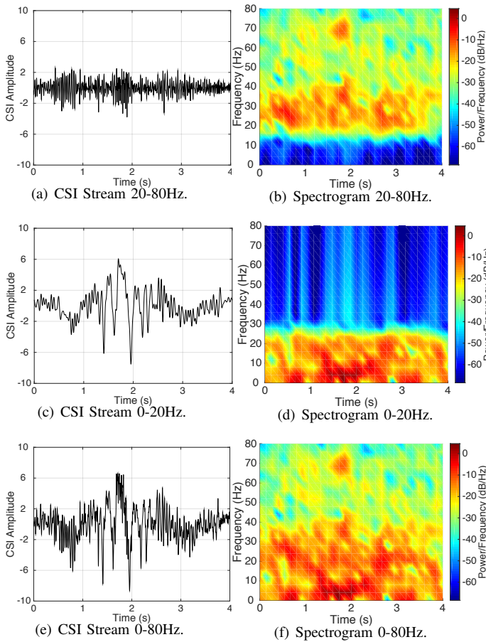
Fig. 4. The three frequency bands of interest. (a)(c)(e) illustrate the CSI stream and (b)(d)(f) show the spectrograms.
