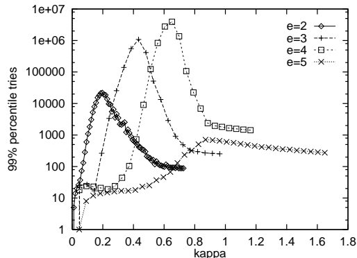
Figure 5: Model B problems with n = 25 and h = 5 , varying number of existentials e , search cost vs. \kappa .
