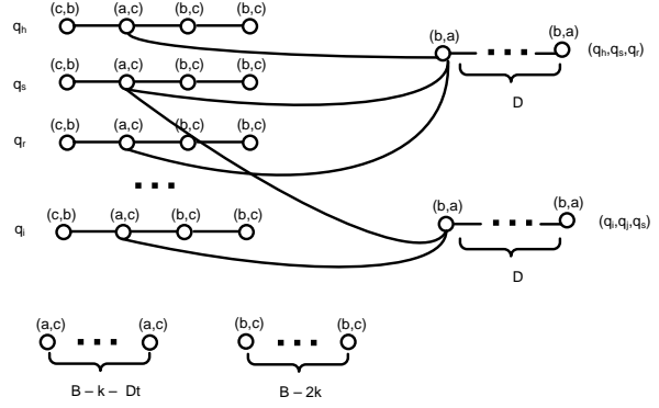
Figure 2: The construction from Theorem 5
