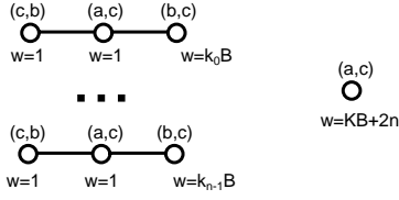
Figure 1: The construction from Theorem 4
