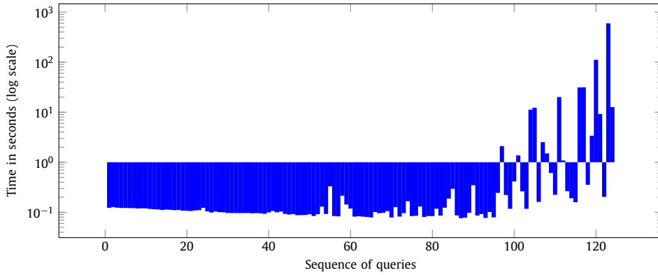
Fig. 3. Time to generate (membership) queries in GenerateQuery.basic on Jigsaw.
