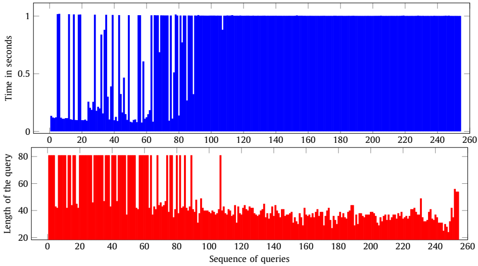
Fig. 4. GenerateQuery.cutoff on Jigsaw : Time to generate queries (top) and their length (bottom).
