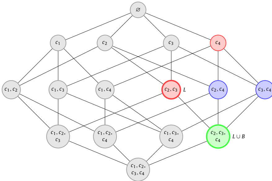
Fig. 1. Comparison of the version spaces of Conacq.2 and QUAcQ2 after processing a positive example e_1^+ and two negative examples e_2^- and e_3^- , violating constraints \{c_1\} , \{c_2, c_4\} , and \{c_3, c_4\} , respectively. After processing e_1^+ , Conacq.2 removes all networks containing c_1 from its version space (grey nodes) because they would reject e_1^+ . Hence, the most specific bound of the version space becomes the green node \{c_2, c_3, c_4\} . When processing the two negative examples e_2^- and e_3^- , Conacq.2 stores two clauses stating that at least one constraint among \{c_2, c_4\} and at least one constraint among \{c_3, c_4\} must belong to the learned network. The most general bound of the version space then becomes the red nodes \{c_4\} and \{c_2, c_3\} . Concerning QUAcQ2 , e_1^+ leads to the removal of c_1 from its bias B , leading to the most specific bound L \cup B = \{c_2, c_3, c_4\} , as in Conacq.2 . When processing e_2^- and e_3^- , thanks to FindScope and FindC , QUAcQ2 learns a unique constraint for each of these two examples, respectively c_2 and c_3 in the figure. This leads to a unique most general bound: the bold red node L = \{c_2, c_3\} in the version space. (For interpretation of the colors in the figure(s), the reader is referred to the web version of this article.)
