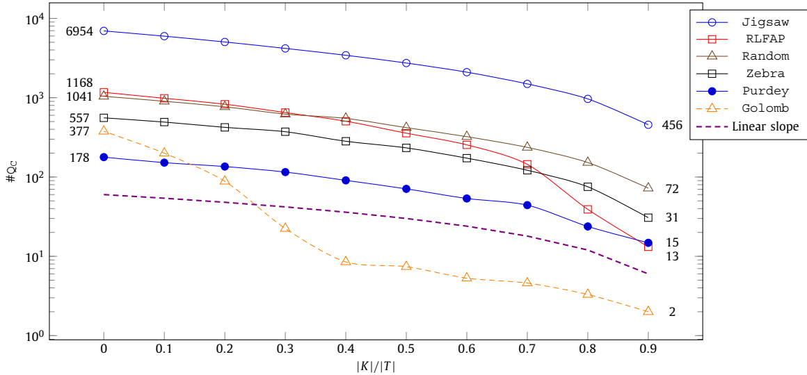
Fig. 5. QuAcQ2.cutoff: Number of queries #Qc when varying the size of the background knowledge K.
