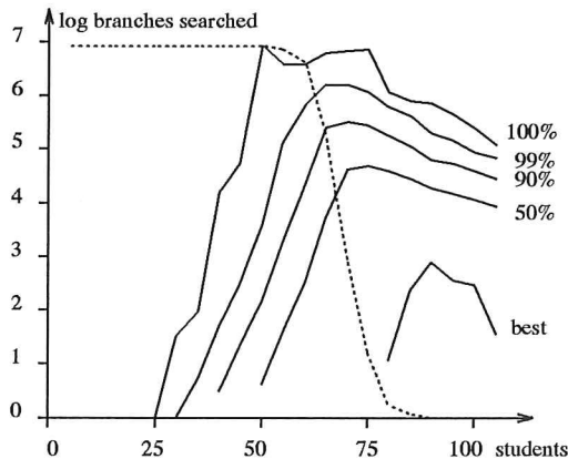
Fig 6: Random time-tables
