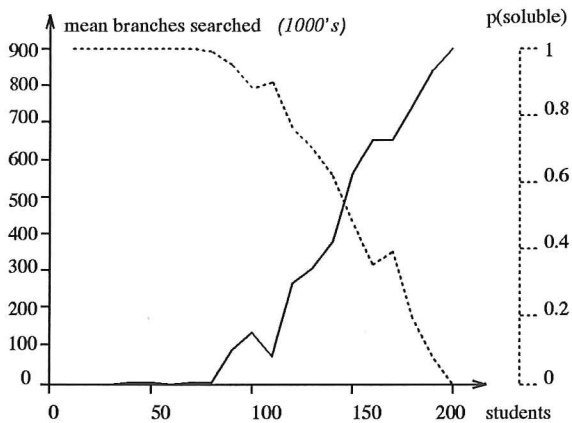
Fig 5: Varying students
