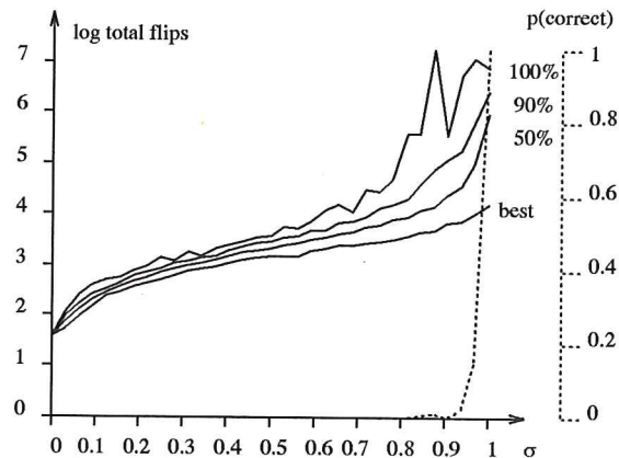
Fig 9: Boolean induction, 2-bit adder
