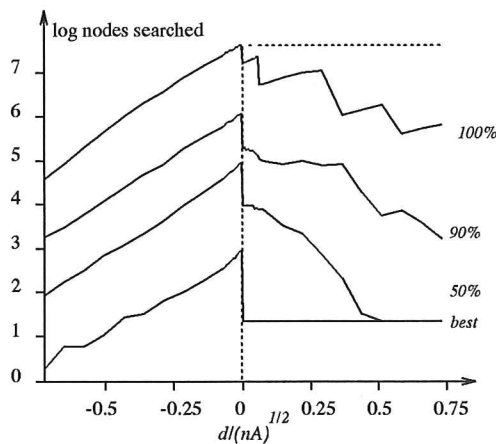
Fig 4: l_{opt} + d for the U.S. capitals
