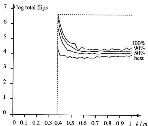
Fig 8: Circuit synthesis, random circuit
