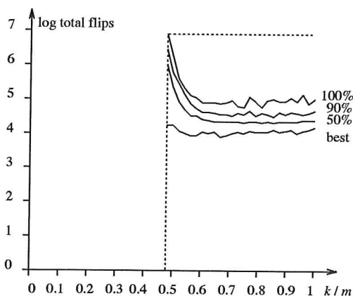
Fig 7: Circuit synthesis, 2-bit adder
