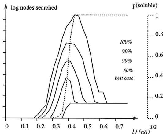
Fig 1: Varying tour length
