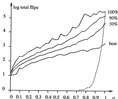
Fig 10: Boolean induction, 3-bit >
