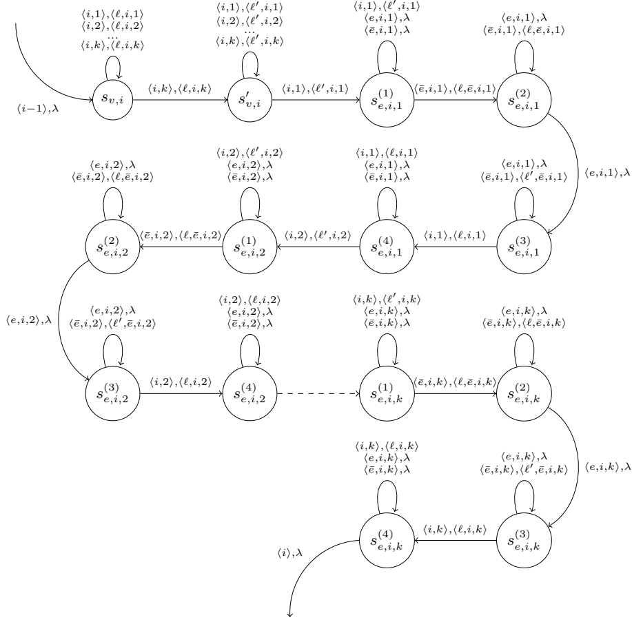
Fig. 1. The i^{\text{th}} part of the Mealy machine M . It does not have the states s_{e,i,i}^{(1)} , s_{e,i,i}^{(2)} , s_{e,i,i}^{(3)} and s_{e,i,i}^{(4)} ; there is instead a transition from s_{e,i,i-1}^{(4)} to s_{e,i,i+1}^{(1)} reading \langle i-1 \rangle and writing \lambda , and there is a transition from s_{e,k,k-1}^{(4)} to a final state reading \langle k \rangle and writing \lambda (drawing all this would have cluttered the figure too much).
