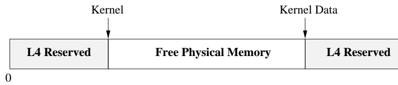
Figure 4.3: Physical Memory Arrangement
