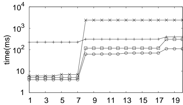
(c) DBLP, DQ15, k = 1 to 20
