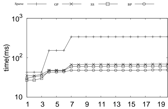
(a) DBLP, DQ11, k = 1 to 20
