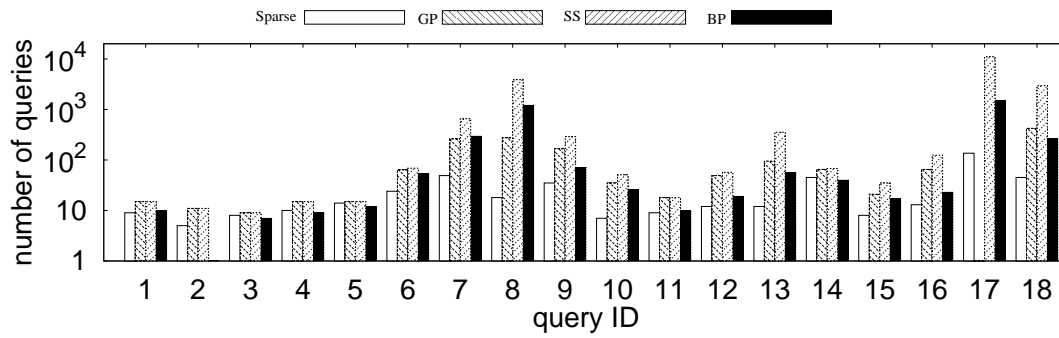
Figure 5.6: Query Number, DBLP, k = 20 , the i -th Query is DQ_i .
