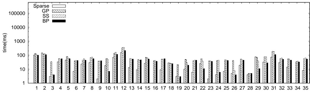
(c) Query Time, Mondial, k = 1
