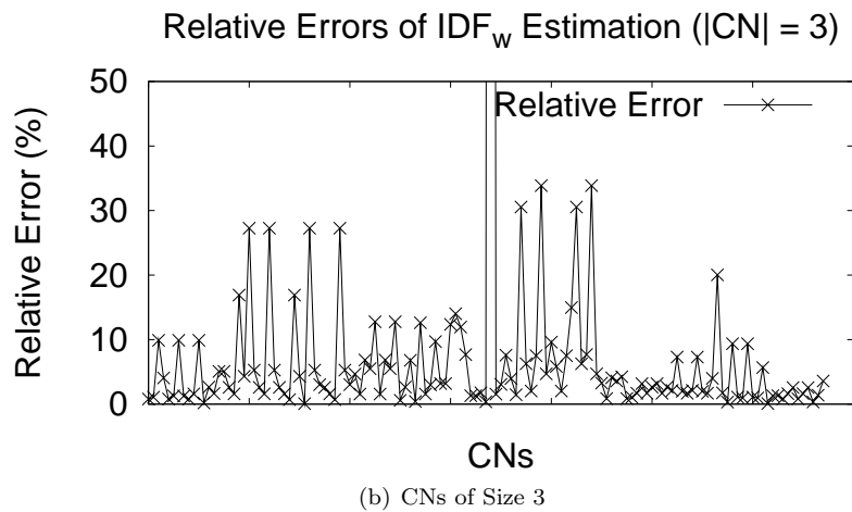
Figure 5.8: Relative Errors of idf_w Estimation
