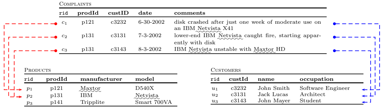
Figure 2.1: A Running Example from [15] (Query is “maxtor netvista”; Matches are Underlined)
