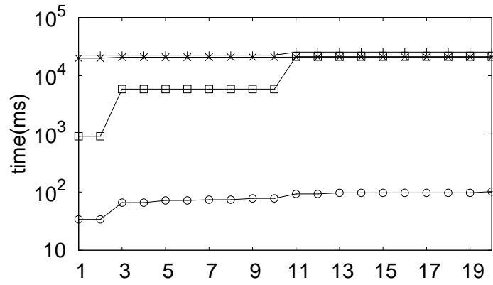
(b) DBLP, DQ13, k = 1 to 20
