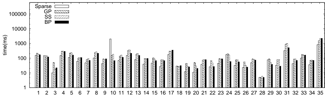
(c) Query Time, Mondial, k = 10 , the i -th Query is MQ_i .
