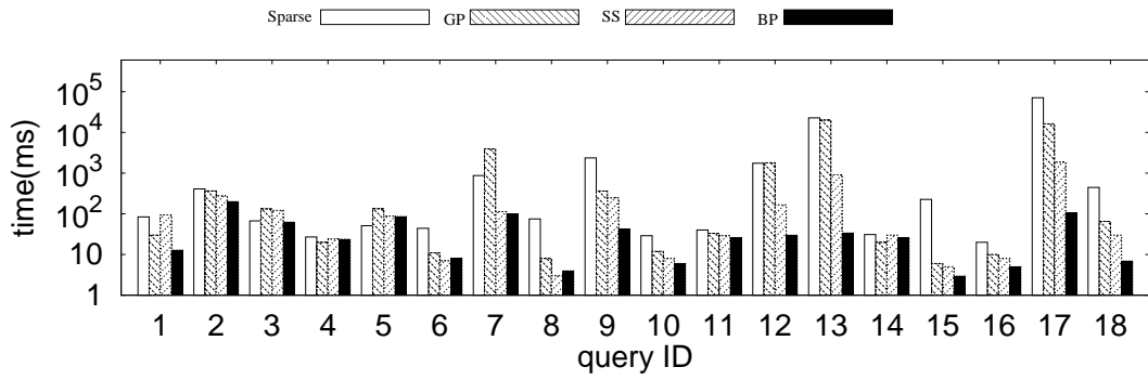
(a) Query Time, DBLP, k = 1 , the i -th Query is DQ_i .
