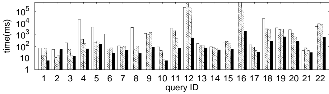
(b) Query Time, IMDB, k = 1 , the i -th Query is IQ_i .
