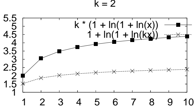
Figure 3.1: Illustrating the Bias when Combining tf Contributions after Attenuation
