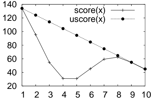
Figure 4.2: Deficiency of Bounding a Non-monotonic Function Using a Monotonic Function
