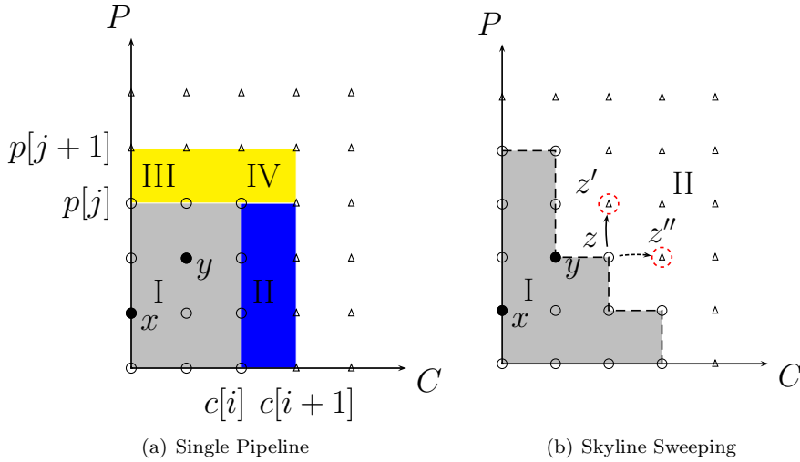
Figure 4.1: Query Evaluation Strategies
