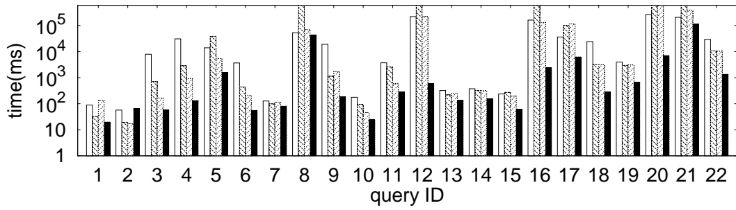
(b) Query Time, IMDB, k = 10 , the i -th Query is IQ_i .
