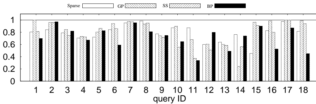
Figure 5.7: Ratio of DBMS Query Processing Time over Overall Elapsed Time, DBLP, k = 20 , the i -th Query is DQ_i .
