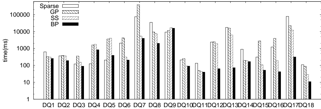
(b) Query Time, DBLP, k = 10
