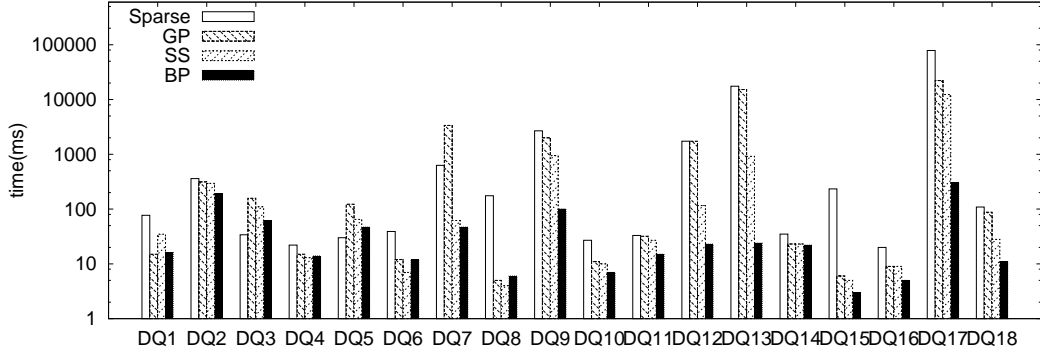
(a) Query Time, DBLP, k = 1
