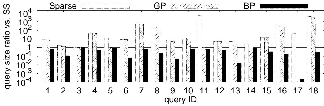
Figure 5.5: Query Size Ratio, DBLP, k = 20 , the i -th Query is DQ_i .
