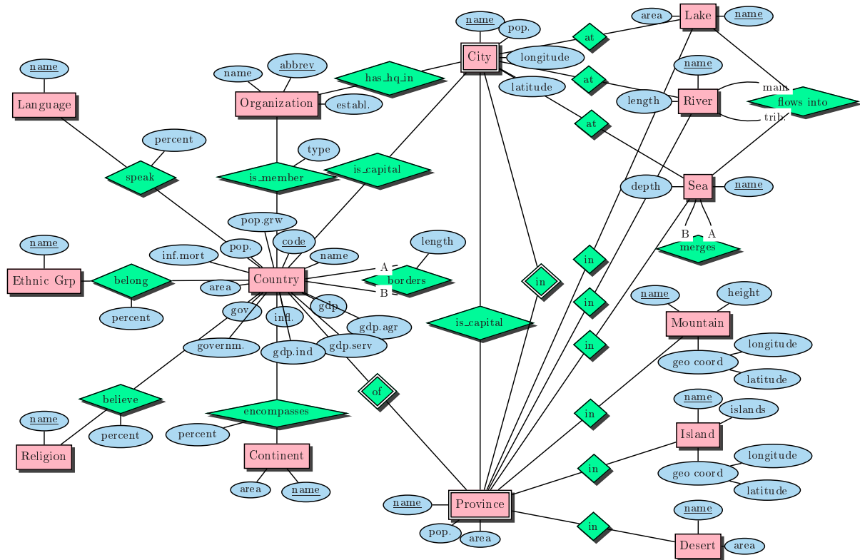
Figure 7.1: ER Diagram For the Mondial Dataset (Original URL: http://www.dbis.informatik.uni-goettingen.de/Mondial/mondial-ER.ps )
