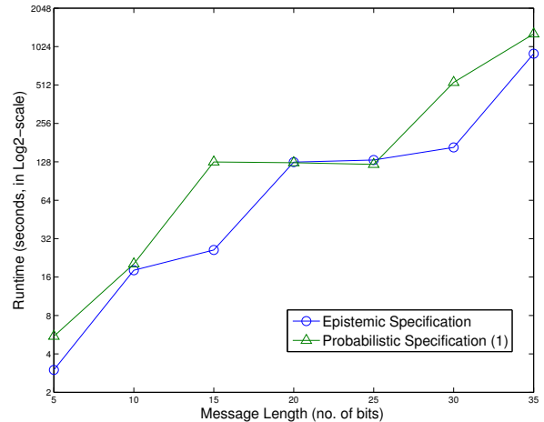
Figure 2: Oblivious Transfer Protocol, Runtime
