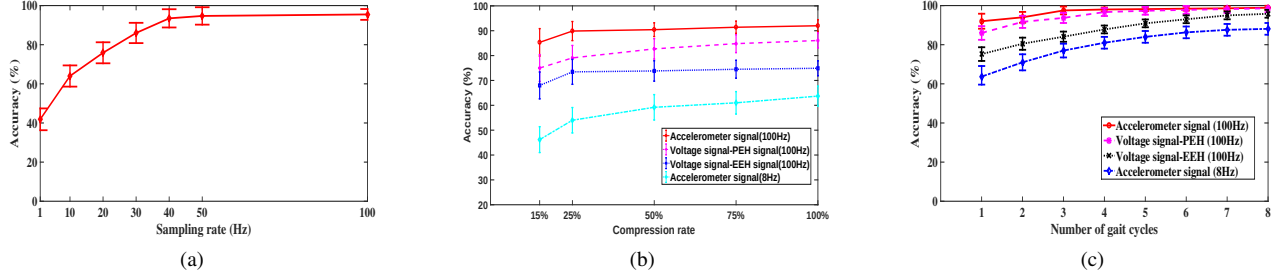
Fig. 11: (a) Recognition accuracy vs sampling rate. (b) recognition accuracy under different compression rate when k=1 . (c) recognition accuracy under different number of gait cycles when = 75\% .
