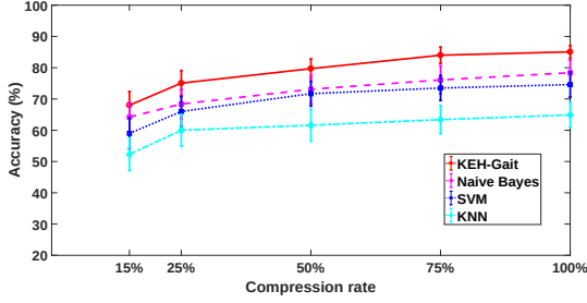
(a) PEH dataset with different compression rate ( k = 1 )
