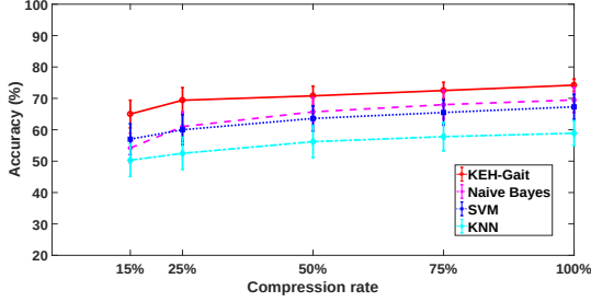
(c) EEH dataset with different compression rate ( k = 1 )
