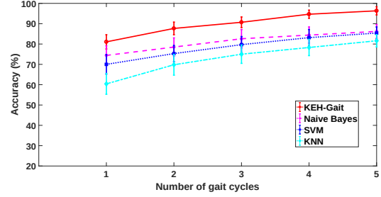
(b) PEH dataset with different k ( \sigma = 0.75 )
