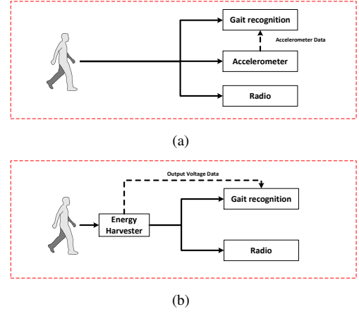
Fig. 3: Gait recognition systems: (a) conventional accelerometer-based gait recognition and (b) KEH-Gait.
