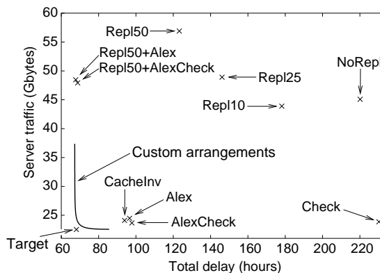
Figure 6: Performance of arrangements vs. one-size-fits-all configurations
