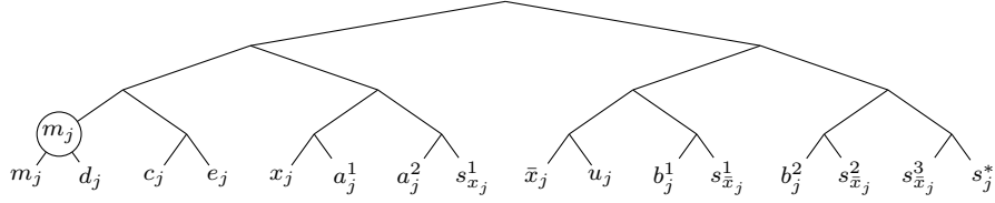
Figure 6: The subtournament for choice gadget j . In this case, x_j = \text{true} is selected.
