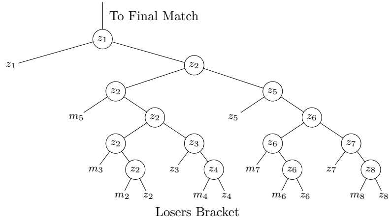
Figure 8: Example of a winners bracket (above) and losers bracket (below) where each left hand player wins each round in their respective ( m and z ) maximal sub-tournaments. The champion of the losers bracket plays the champion of the winners bracket in a final match.
