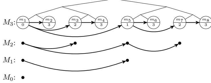
Figure 1: The spawning process for the case k = 8 , the lower part of each node shows the corresponding value of l_j . By the draw shown on top of M_3 , the leftmost player can win the BKT.
