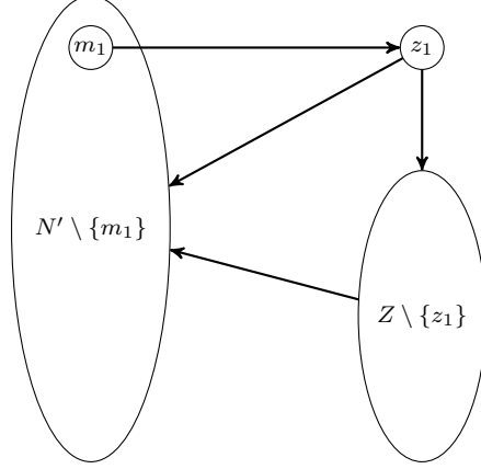
Figure 7: Pairwise comparison among members of the set N from Lemma 5.
