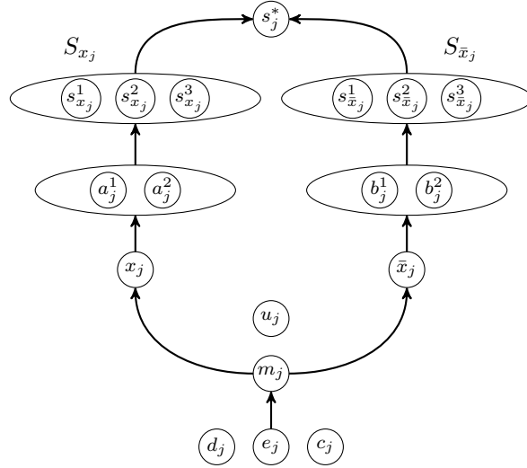
Figure 3: Pairwise comparisons in the j -th choice gadget. All arrows not shown in the figure run downwards, horizontal arcs run right to left. Vertices grouped in a component have the same relation with vertices outside the component.
