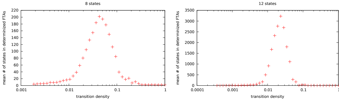
Figure 1: Graphs plotting the mean size of the determinized FTAs obtained by determinization over the density for FTAs of size 8 and 12. Minimization reduces the mean size, but does not move the peak.
