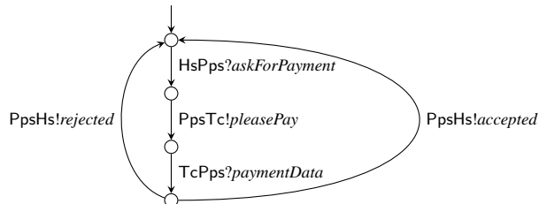
(c) Communicating machine for the port PPS
