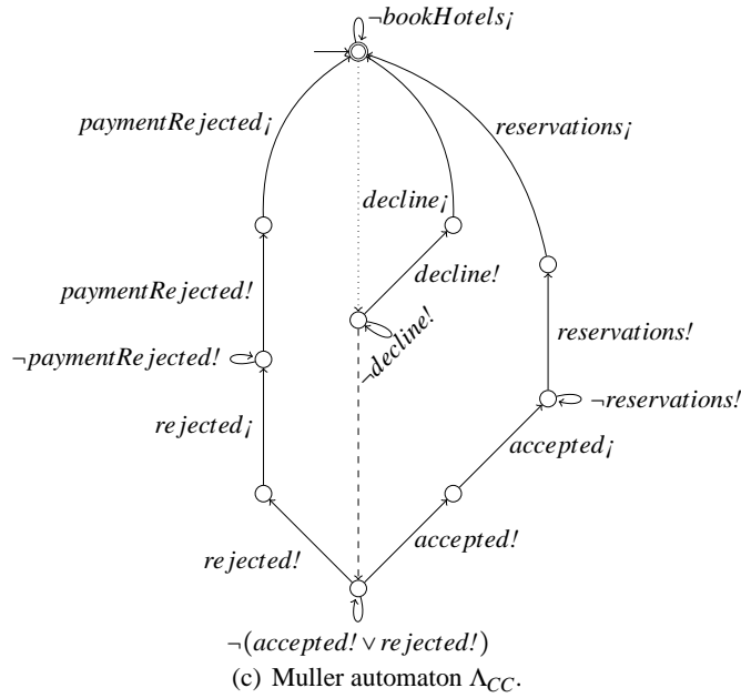
Figure 1: The TravelClient activity together with the Muller automata.
