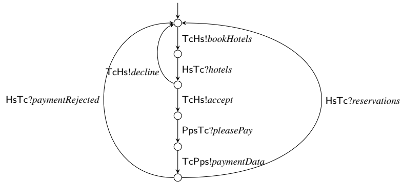
(a) Communicating machine for the port TC
