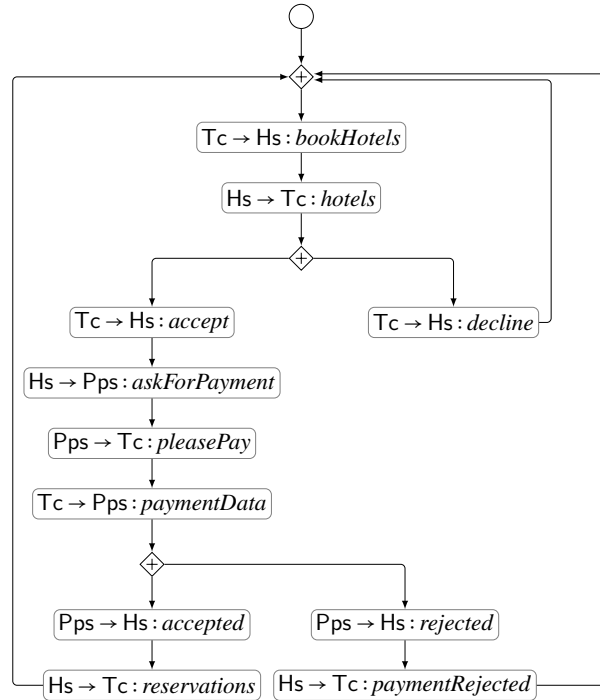
Figure 5: Global graph of the running example
