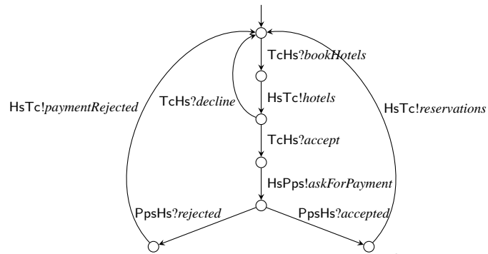
(b) Communicating machine for the port HS
