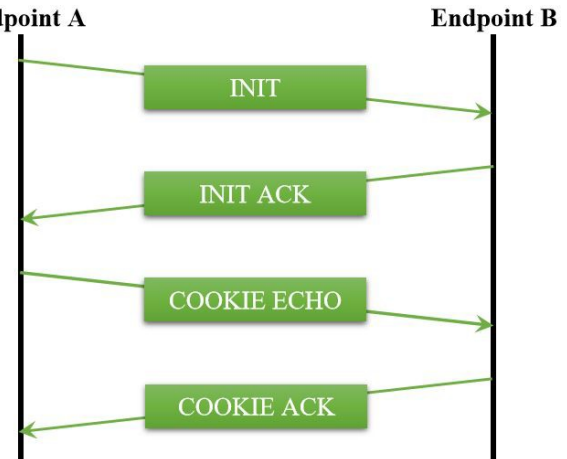
Figure 5: SCTP four-way handshake
