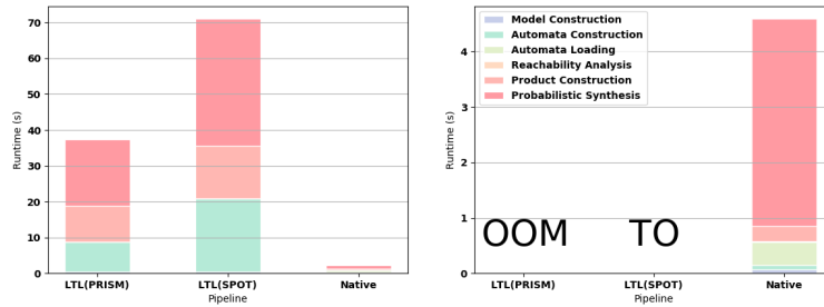
(a) 200-height random Nim game.
