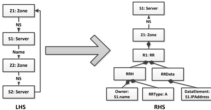
Figure 7: Refactoring Rule: AddGlueRecord.
