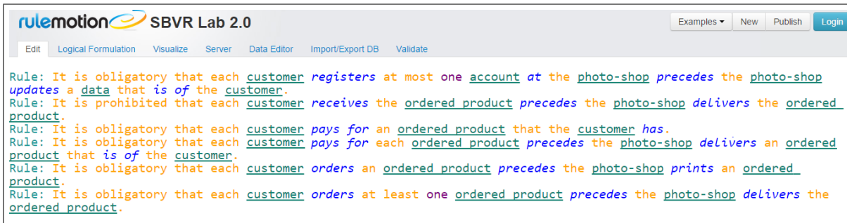
Figure 4: Rules in the Online Photo Shop case study
