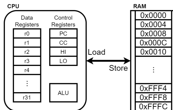
Figure 2: A Simple CPU
