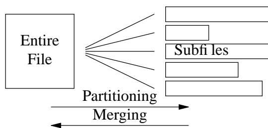
Figure 23. Partitioning Skew.
