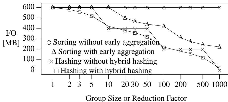
Figure 14. Performance of Sort- and Hash-Based Aggregation.
