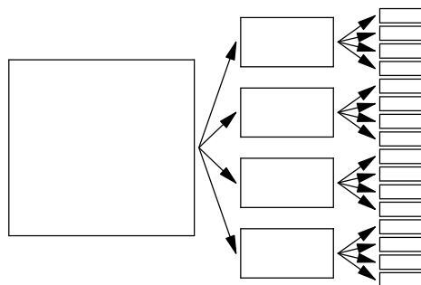
Figure 10. Recursive Partitioning.
