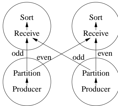
Figure 38. Deadlock-Free Scenario.
