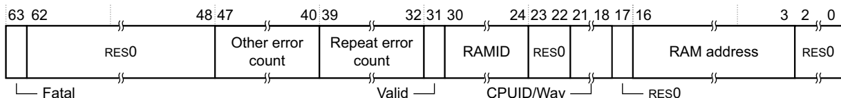
Figure 4-74 L2MERRSR_EL1 bit assignments
