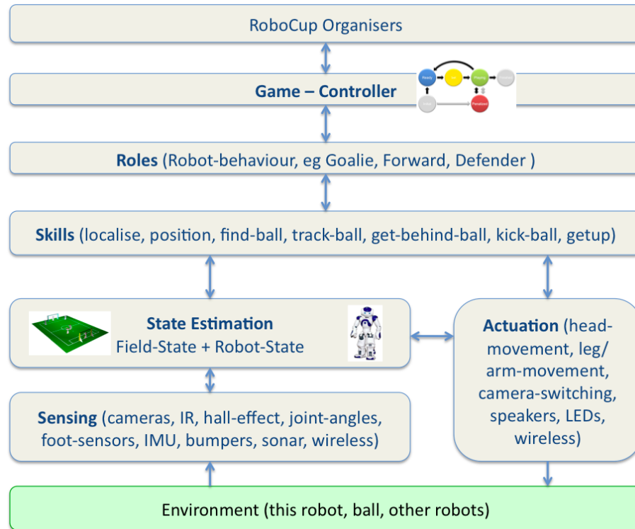
Fig. 1. The 2012 UNSW SPL robotic architecture.
