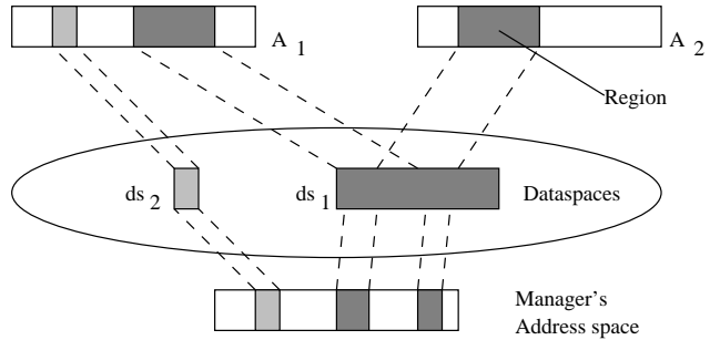
Figure 4. Relationship between address spaces, dataspaces, and regions.
